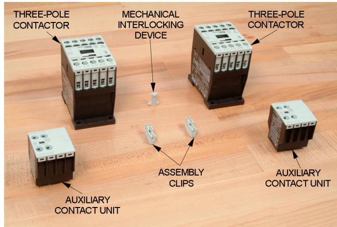
Figure 3-10. Mechanical interlocking.
